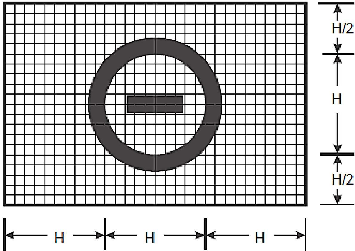
Figure APP.D-4: NO ENTRY sign
