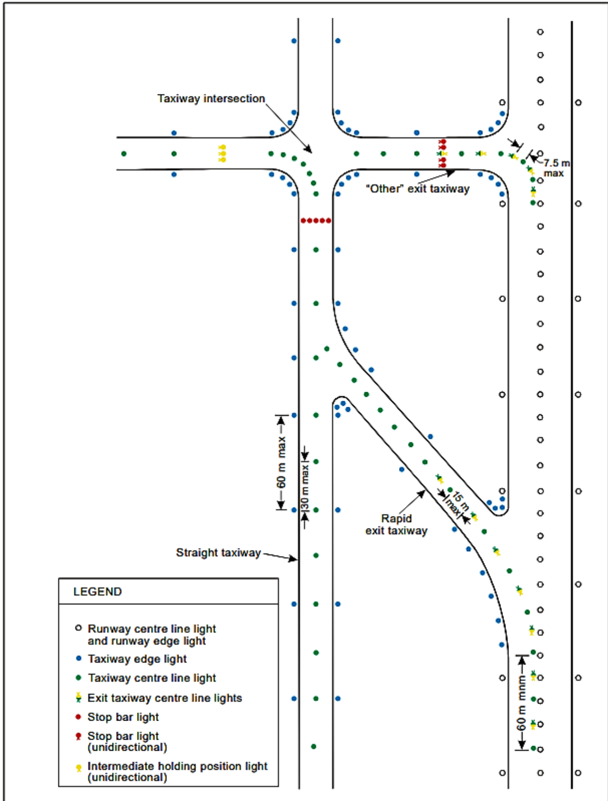
Figure 28: Taxiway lighting
