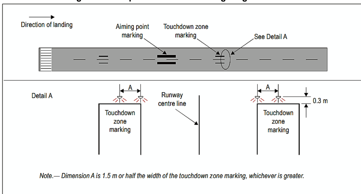
Figure 30: Simple touchdown zone lighting
