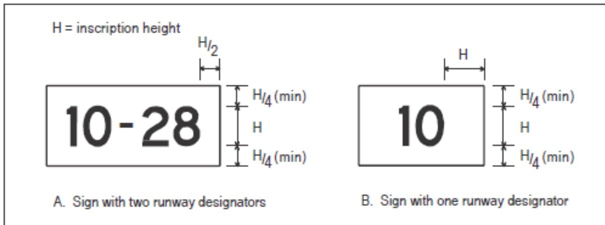
Figure APP.D-5: Sign dimensions
