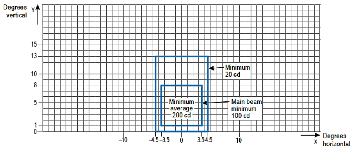
Figure APP.B-13: Isocandela diagram for taxiway centre line (15 m spacing), no-entry bar, and stop bar lights in straight sections intended for use in RVR of less than a value of 300 m
