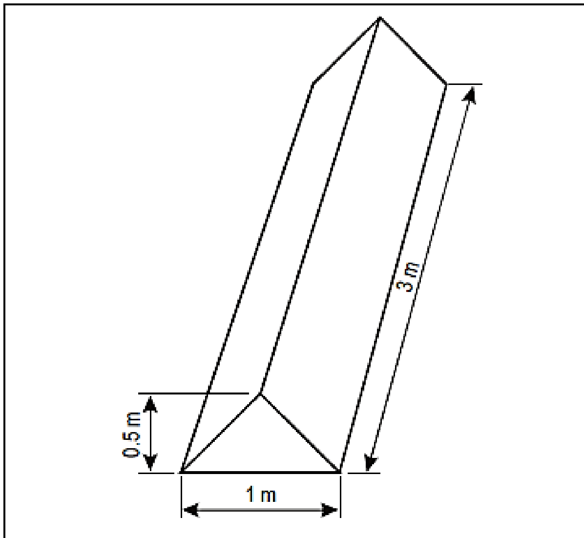
Figure 42: Boundary markers
