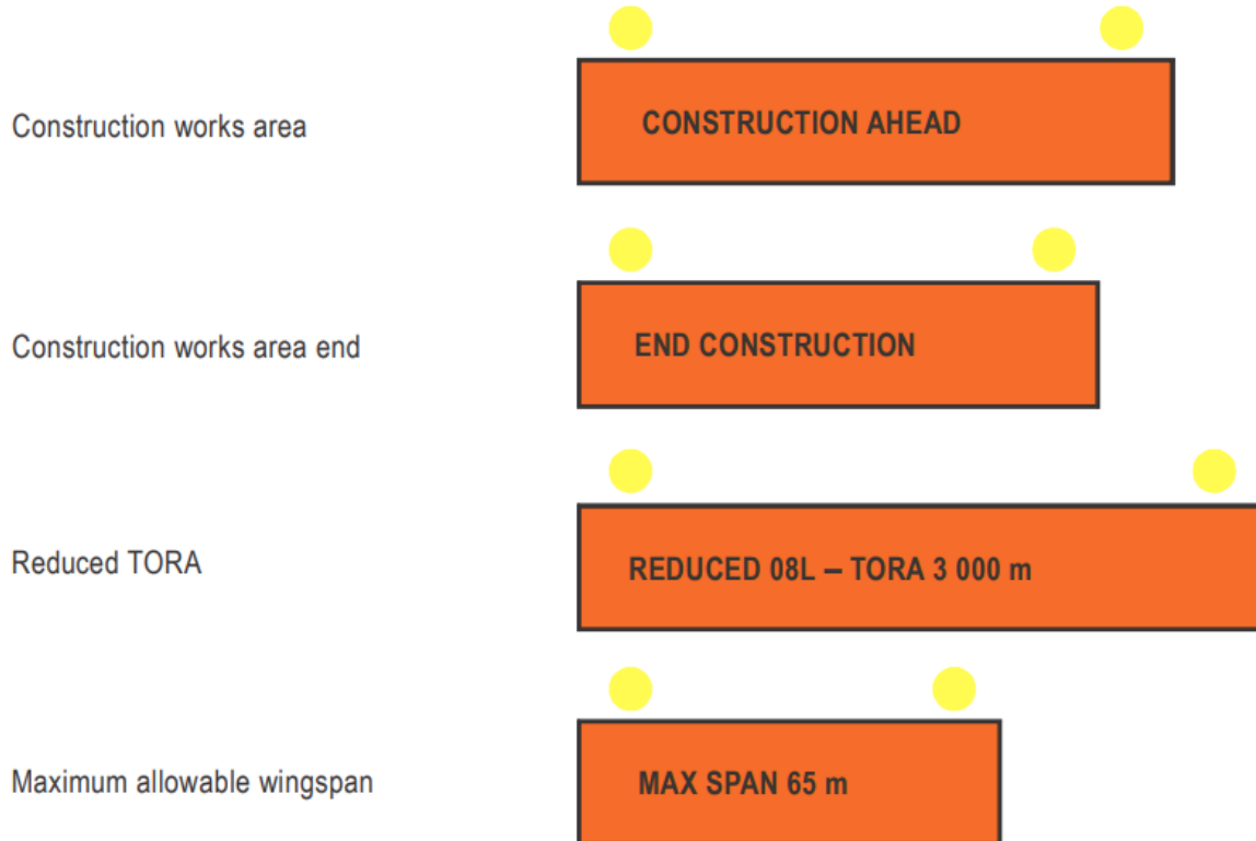
Figure 47: Examples of unserviceability signs
