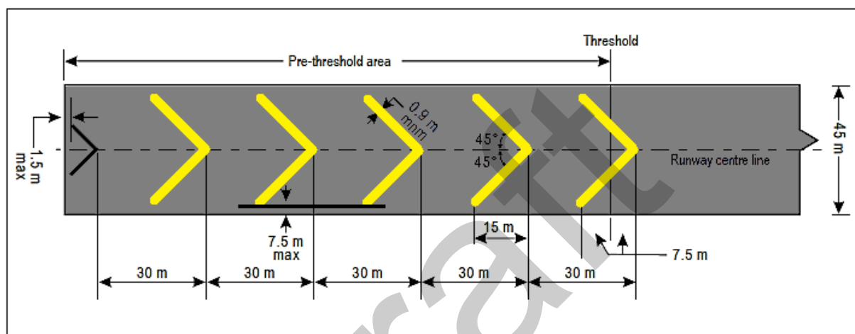
Figure 39: Pre-threshold marking
