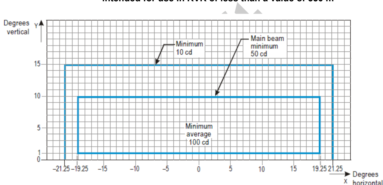
Figure APP.B-14: Isocandela diagram for taxiway centre line (7.5 m spacing), RELs, no-entry bar, and stop bar lights in curved sections intended for use in RVR of less than a value of 350 m
