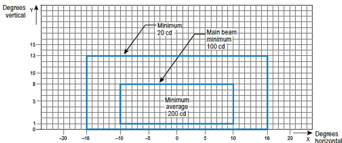
Figure APP.B-12: Isocandela diagram for taxiway centre line (15 m spacing), RELs, no-entry bar, and stop bar lights in straight sections intended for use in RVR of less than a value of 350 m where large offsets can occur and for low-intensity runway guard lights, Configuration B
