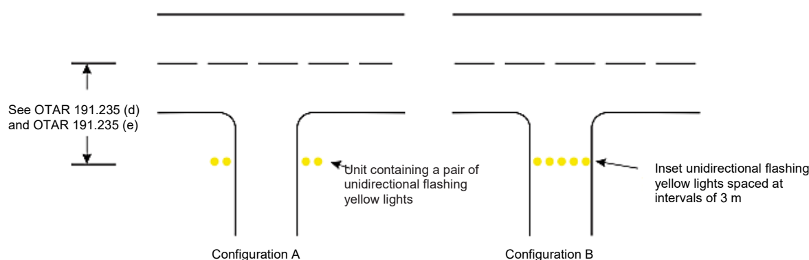
Figure 35: Runway guard lights
