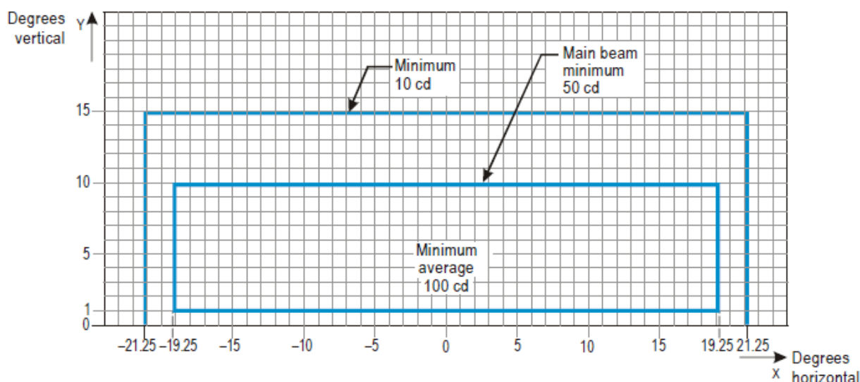
Figure APP.B-14: Isocandela diagram for taxiway centre line (7.5 m spacing), RELs, no-entry bar, and stop bar lights in curved sections intended for use in RVR of less than a value of 350 m
