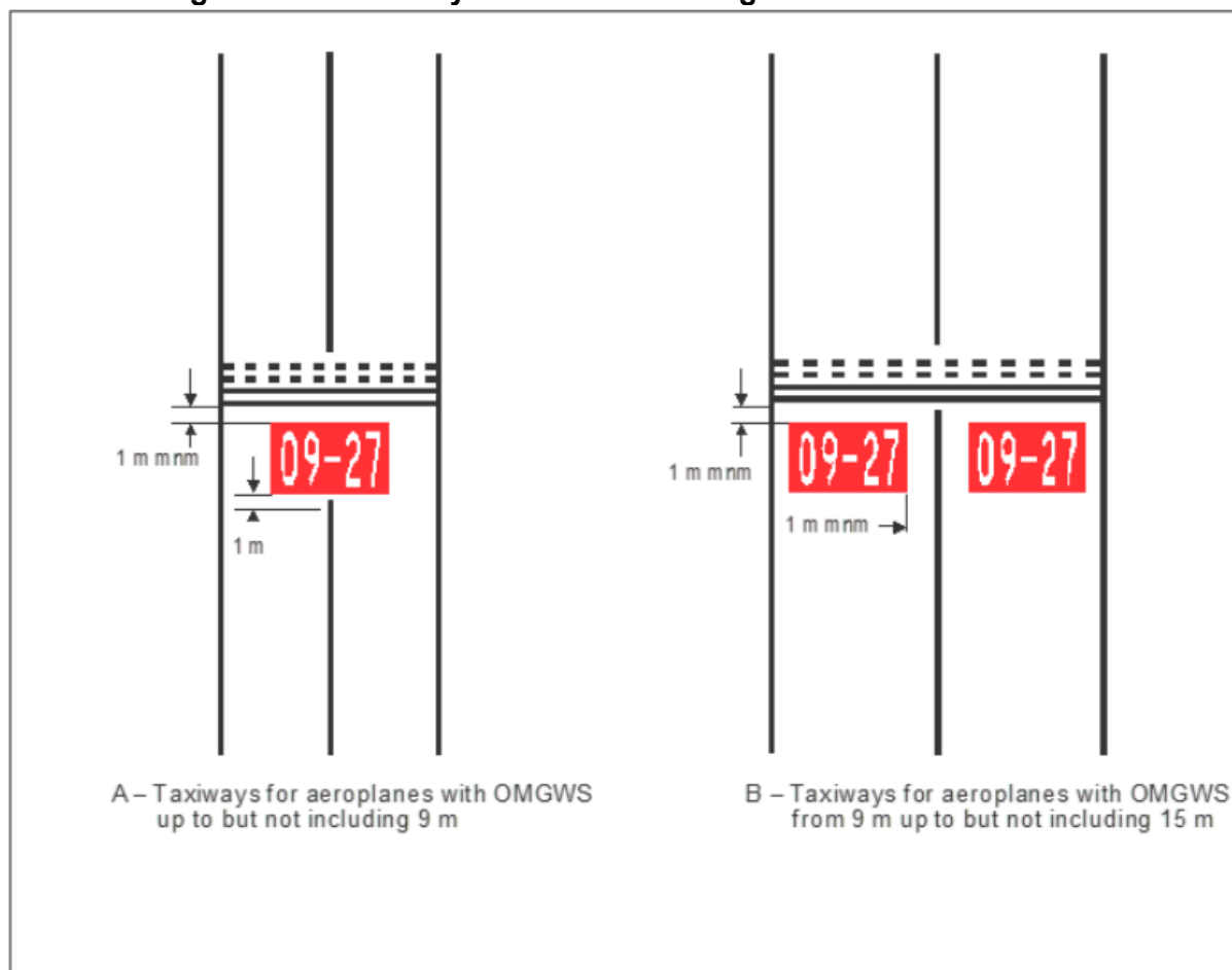
Figure 18. Mandatory instruction marking
