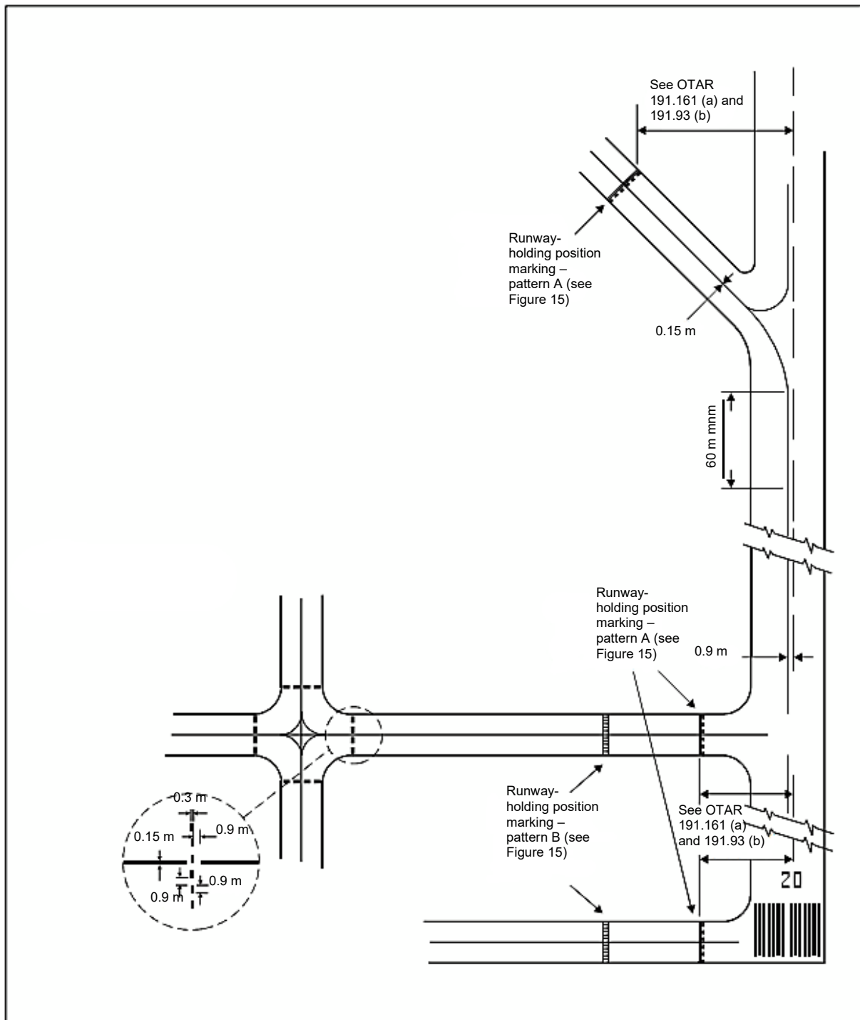
Figure 13. Taxiway markings (shown with basic runway markings)
