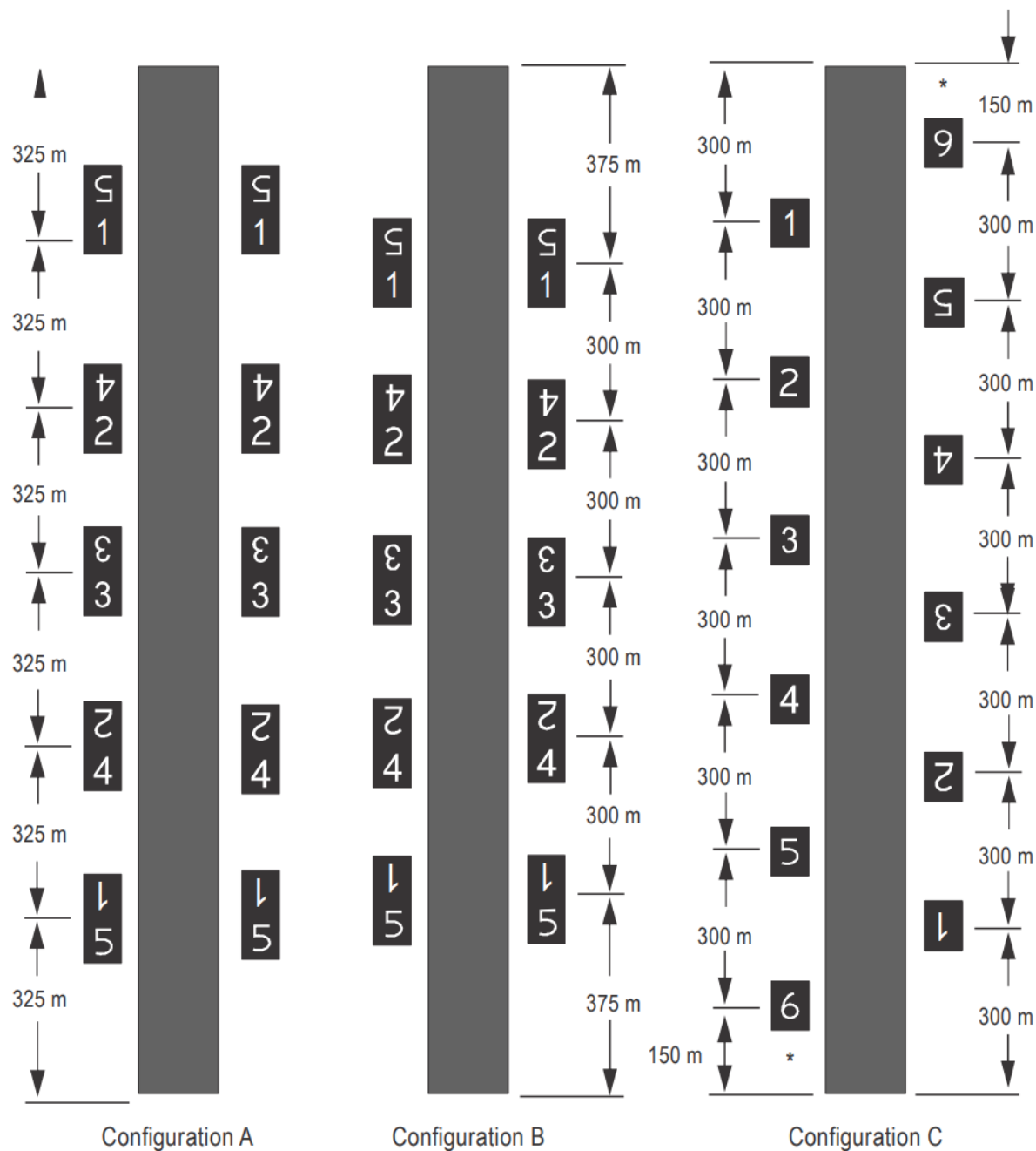
Figure APP.D-7: Runway distance remaining sign configurations
