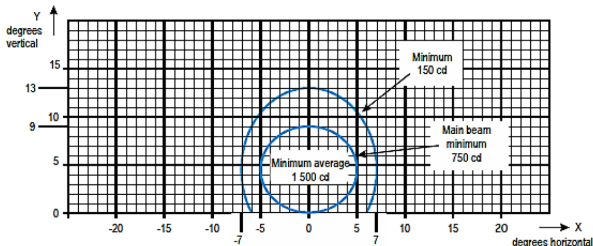
Figure APP.B-25: Isocandela diagram for take-off and hold lights (THL) (red light)
