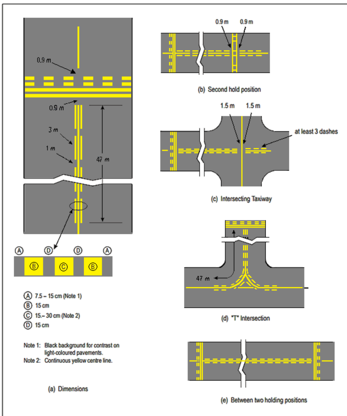
Figure 14: Enhanced taxiway centre line marking
