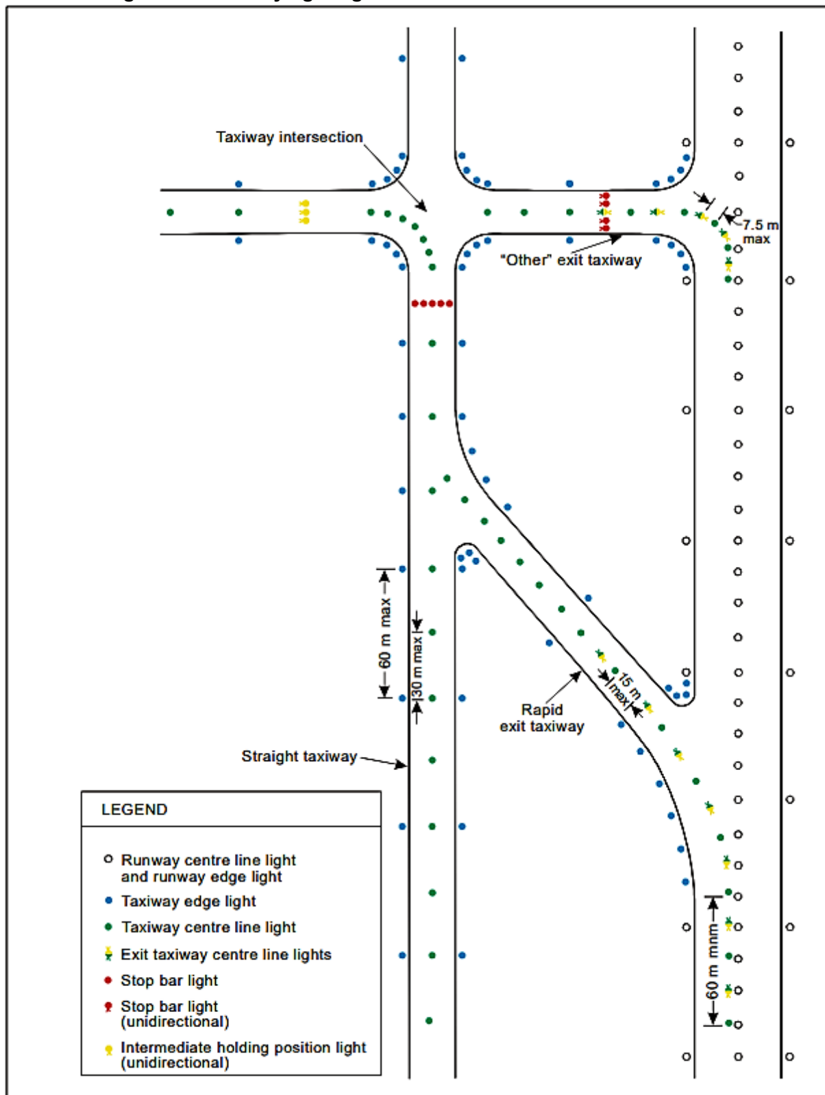
Figure 28: Taxiway lighting
