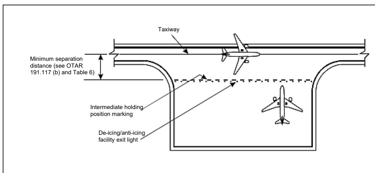
Figure 34: Typical remote de-icing/anti-icing facility
