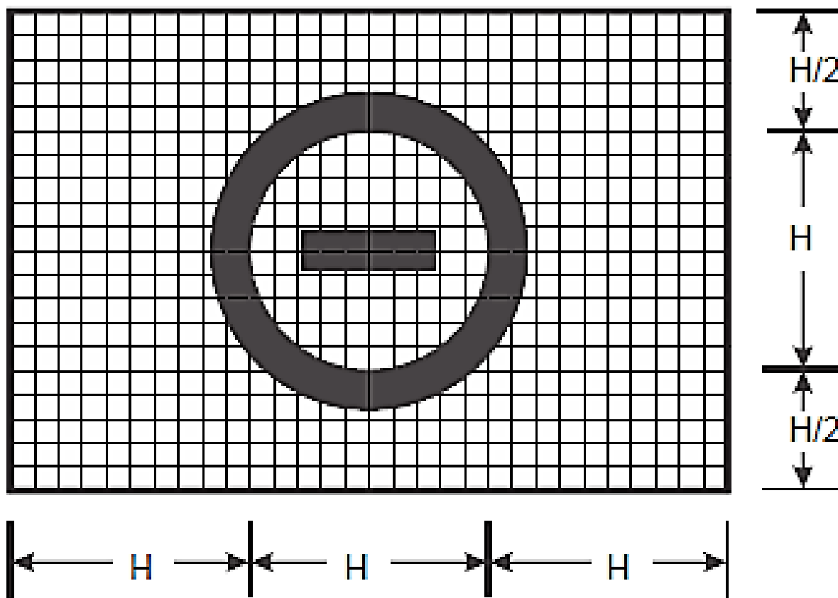
Figure APP.D-4: NO ENTRY sign
