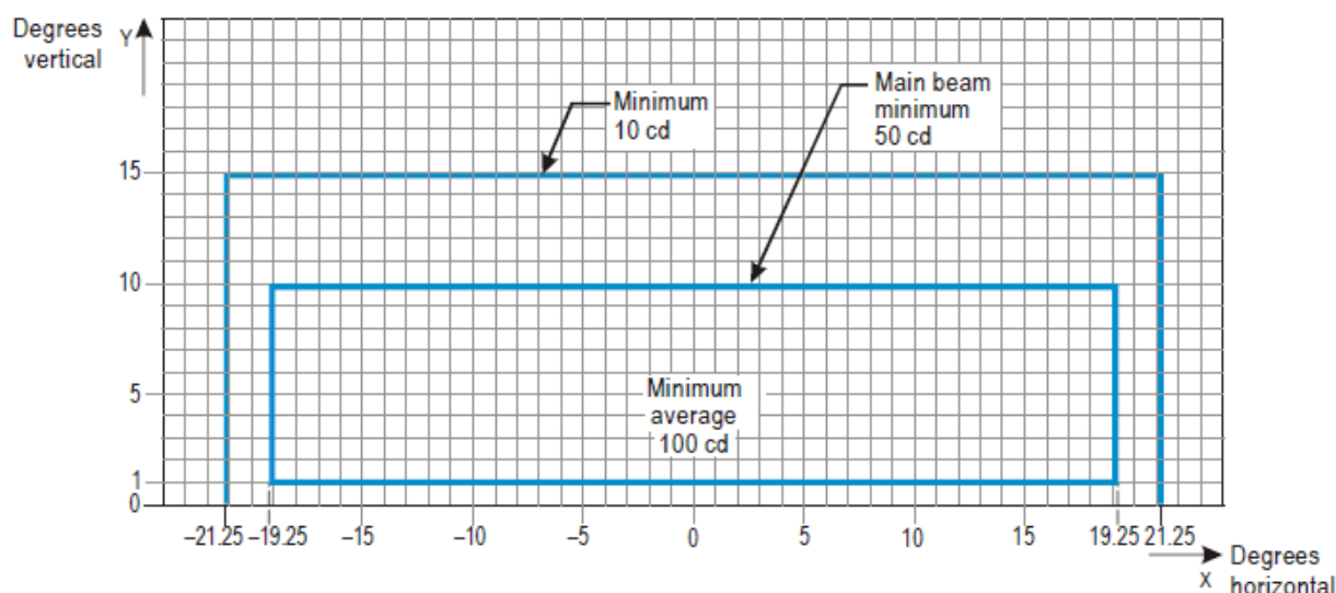
Figure APP.B-14: Isocandela diagram for taxiway centre line (7.5 m spacing), RELs, no-entry bar, and stop bar lights in curved sections intended for use in RVR of less than a value of 300 m
