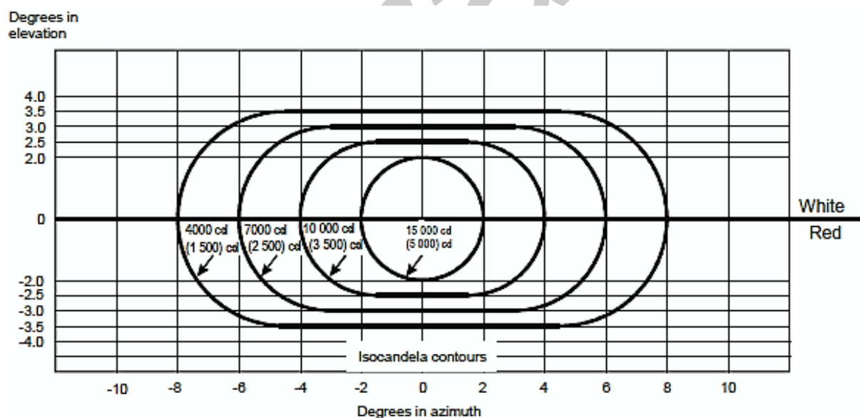
Figure APP.B-22: Light intensity distribution of PAPI and APAPI
