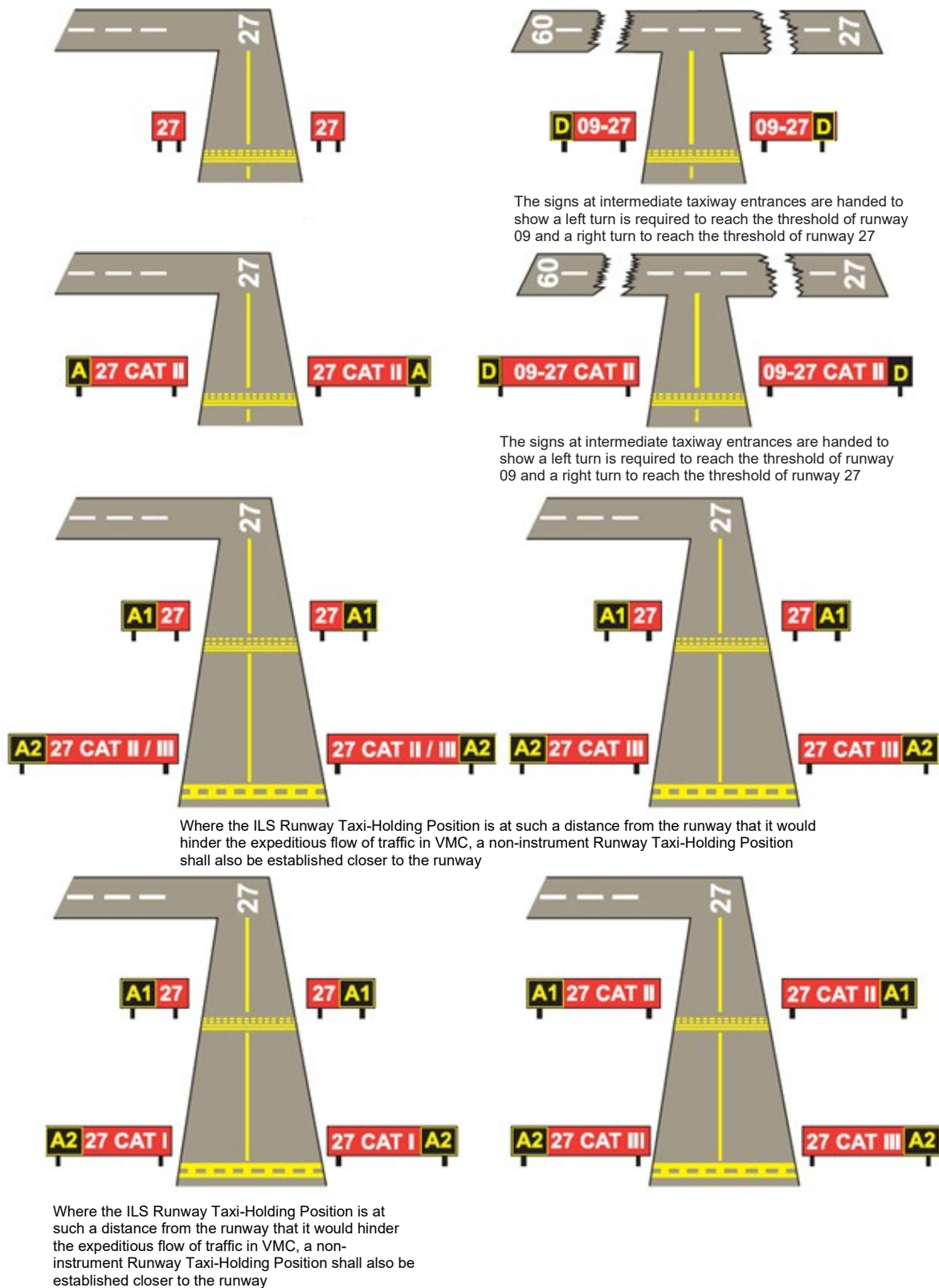
Figure 17: Typical runway taxi-holding position signs and associated taxiway marking
