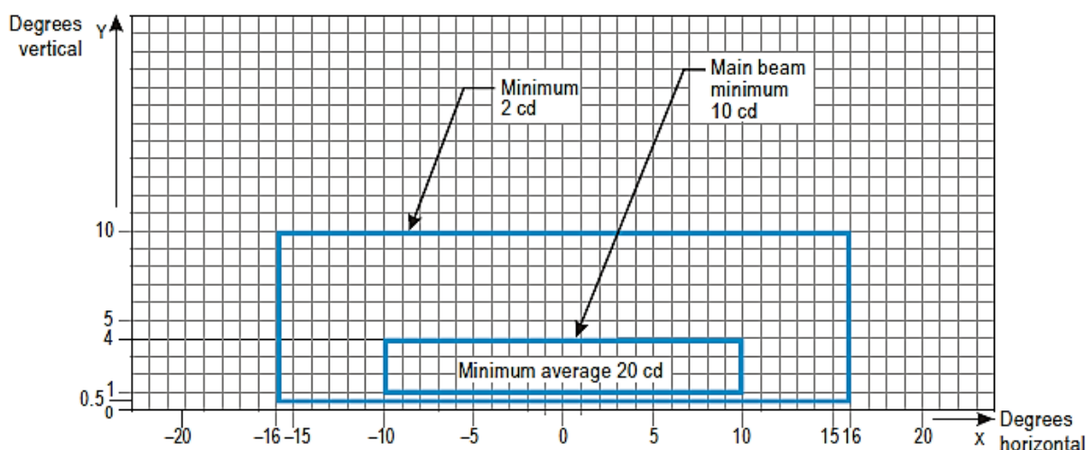
Figure APP.B-15: Isocandela diagram for taxiway centre line (30 m, 60 m spacing), no-entry bar and stop bar lights in straight sections intended for use in RVR of 300 m or greater
