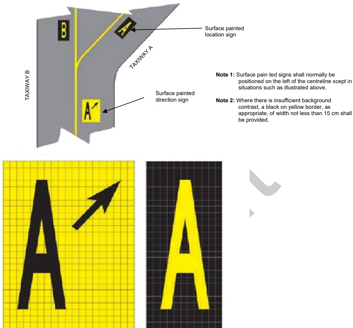
Figure APP.C-6: Pavement markings for taxiways and aprons – examples of surface-painted signs
