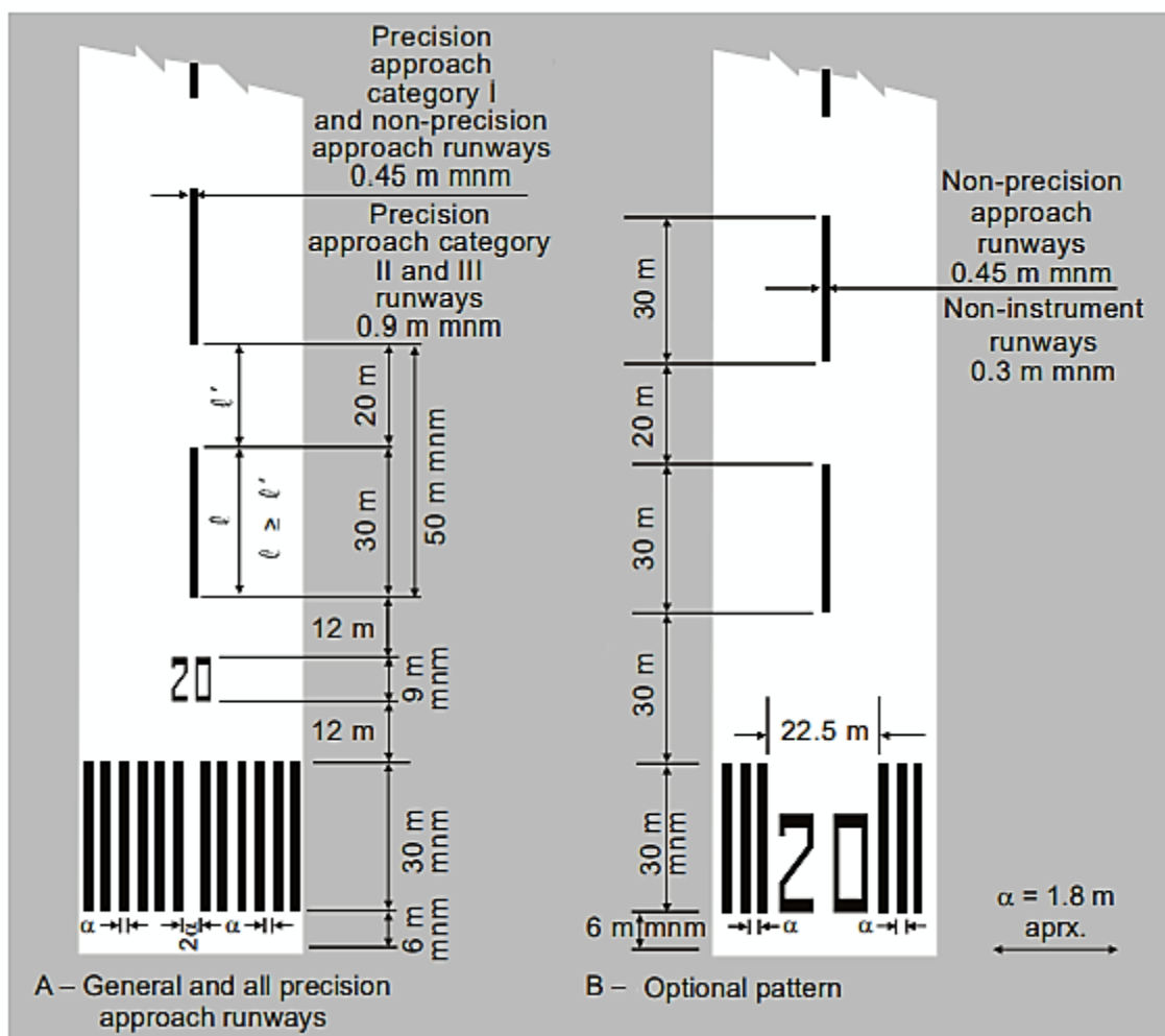
Figure 9. Runway designation, centre line and threshold markings
