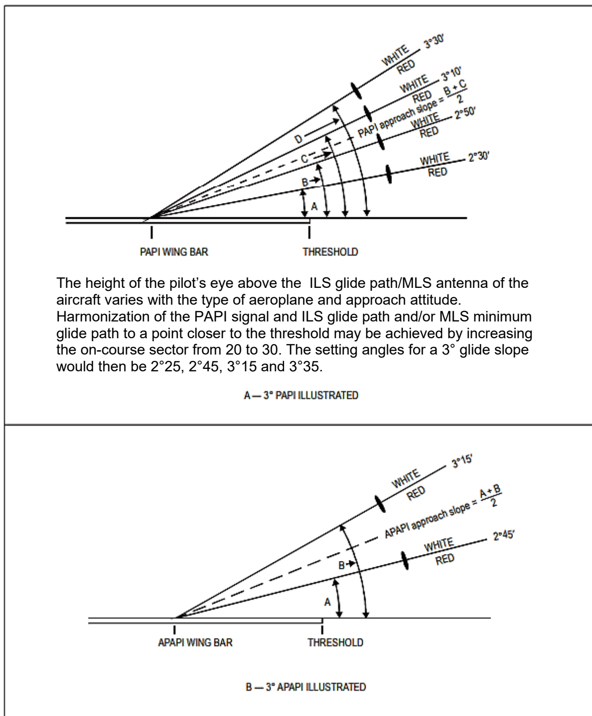
Figure 26: Light beams and angle of elevation setting of PAPI and APAPI
