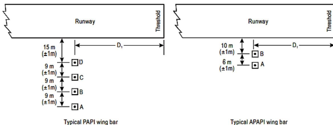
Figure 25: Location of PAPI and APAPI
