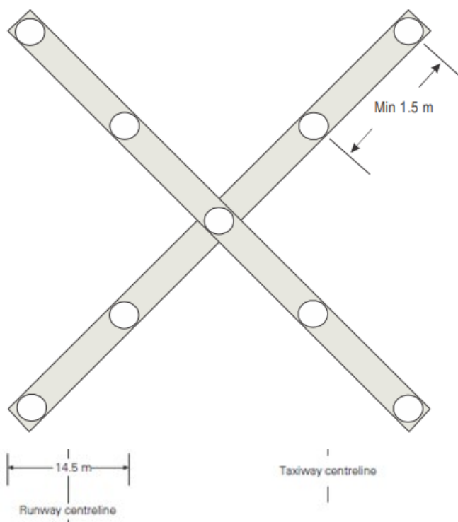
Figure 46: Example of elevated closed runway lighting – five lights per branch | Figure 45: Closed runway and taxiway markings
