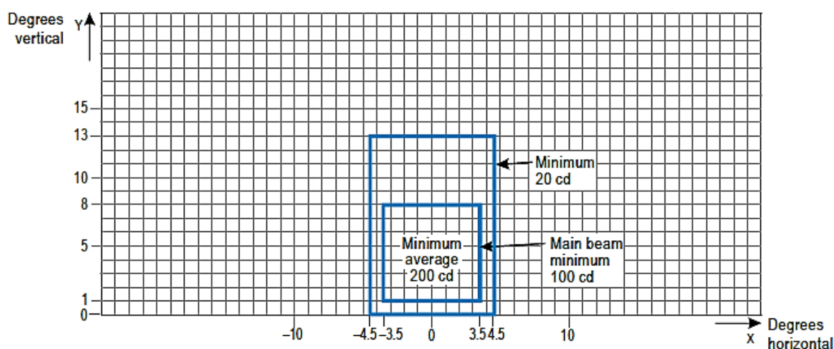
Figure APP.B-13: Isocandela diagram for taxiway centre line (15 m spacing), no-entry bar, and stop bar lights in straight sections intended for use in RVR of less than a value of 300 m
