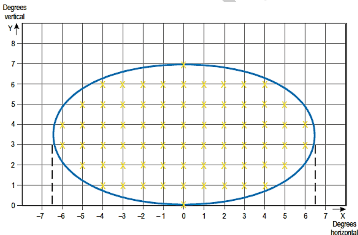
Figure APP-B.11: Grid points to calculate the average intensity of approach and runway lights.
