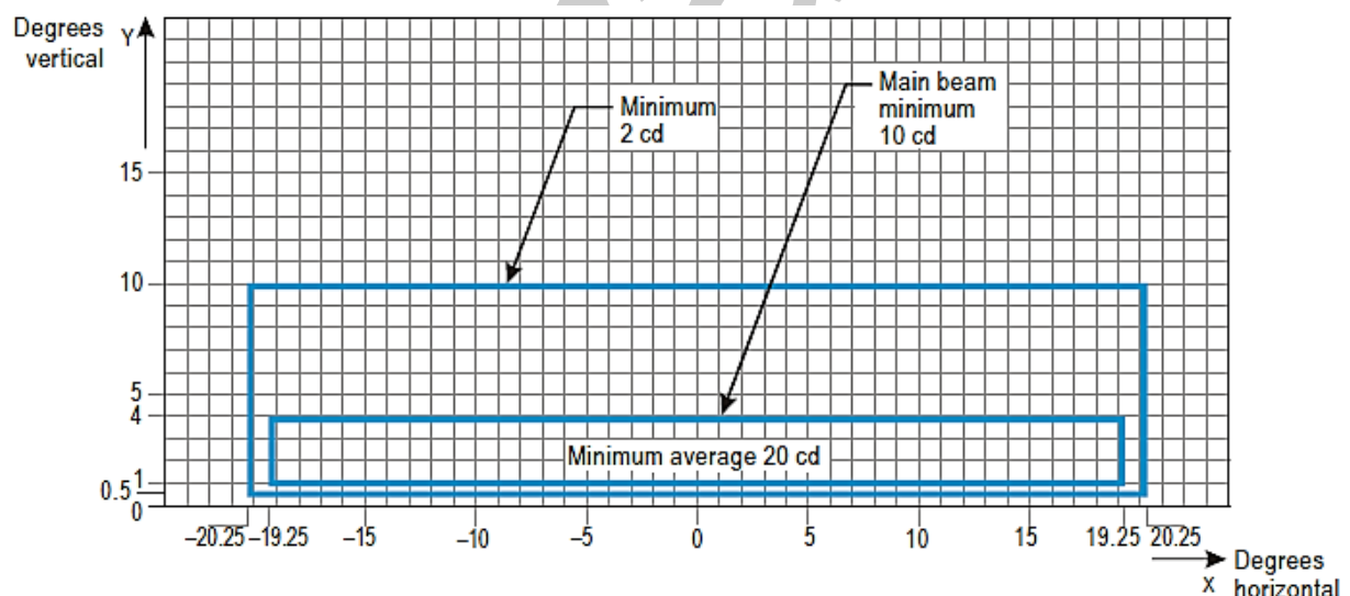
Figure APP-B.16: Isocandela diagram for taxiway centre line (7.5 m, 15 m, 30 m spacing), no-entry bar and stop bar lights in curved sections intended for use in RVR of 300 m or greater
