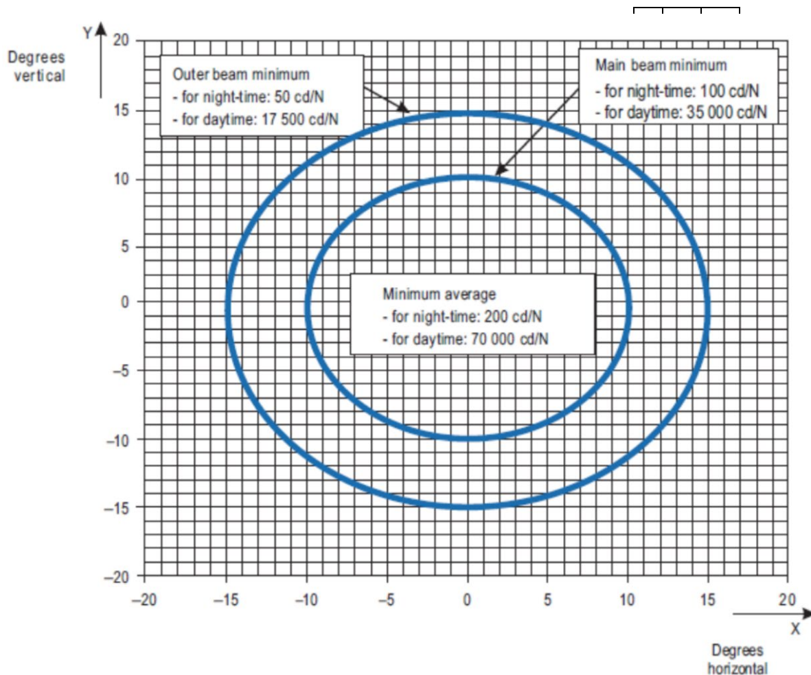
Figure APP.B-26: Isocandela diagram for closed runway lights (white light)
