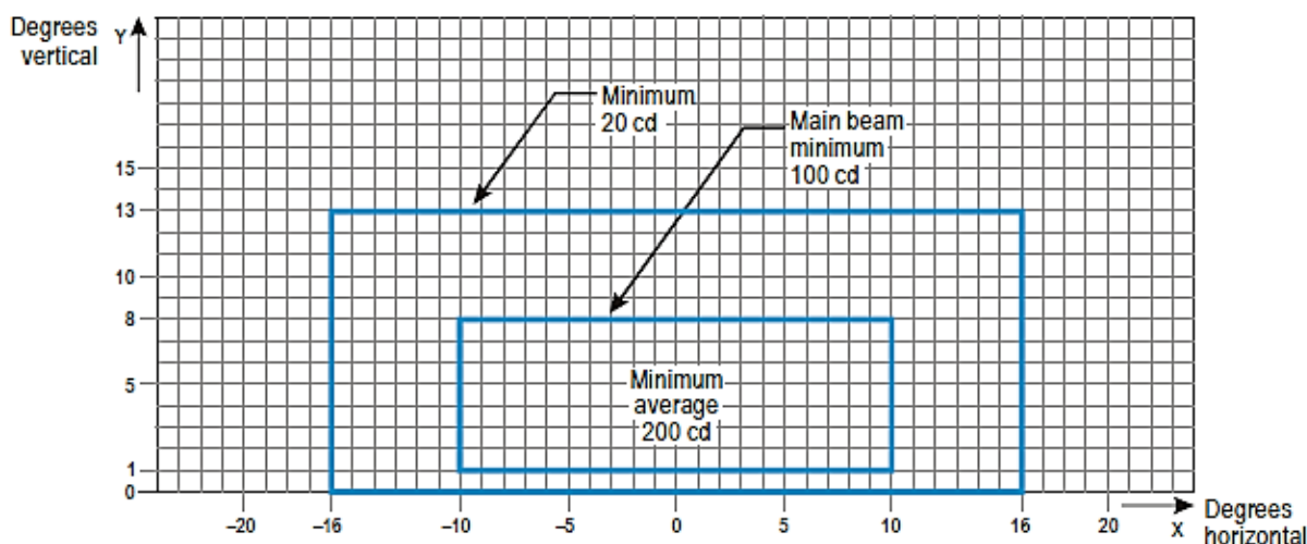
Figure APP.B-12: Isocandela diagram for taxiway centre line (15 m spacing), RELs, no-entry bar, and stop bar lights in straight sections intended for use in RVR of less than a value of 300 m where large offsets can occur and for low-intensity runway guard lights, Configuration B
