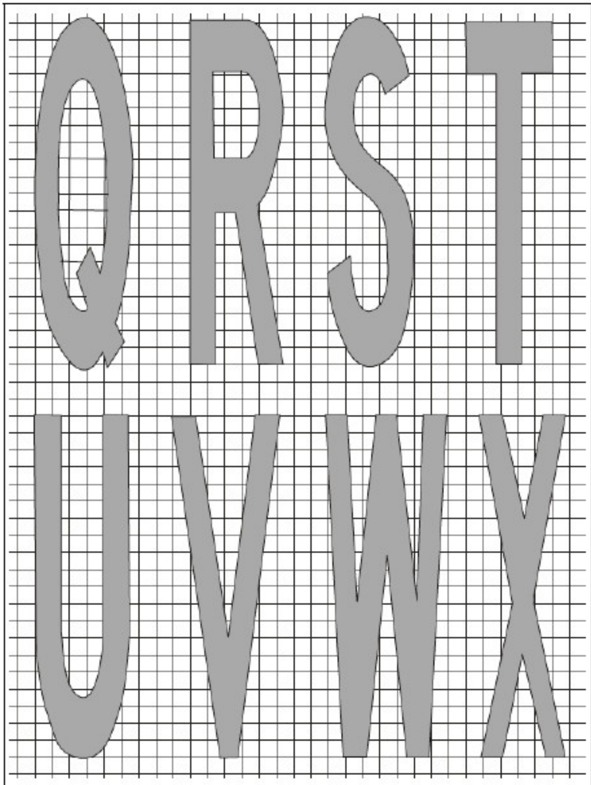
Figure APP.C-4: Mandatory instruction markings (cont.)
