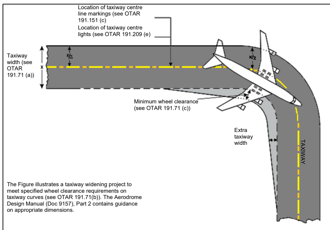
Figure 2: Taxiway curve
