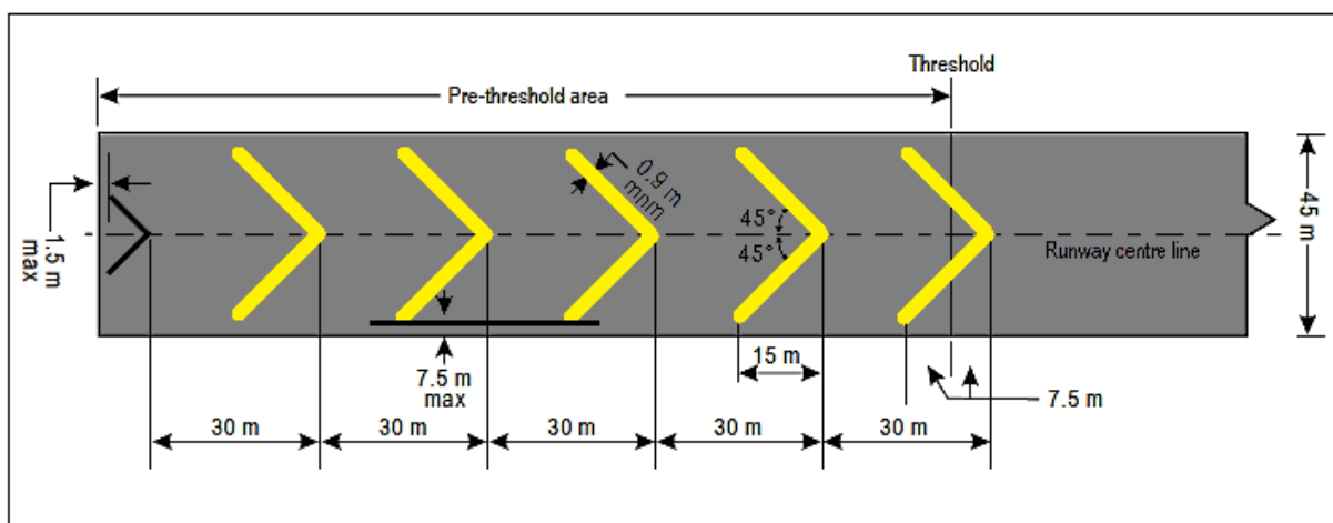
Figure 39: Pre-threshold marking
